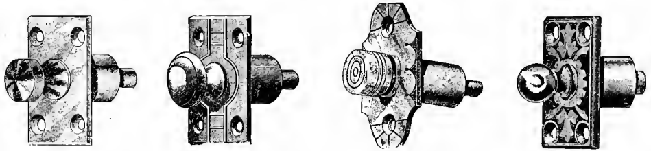
Figs. 4465-4468. END-DOOR-SASH BOLTS.
